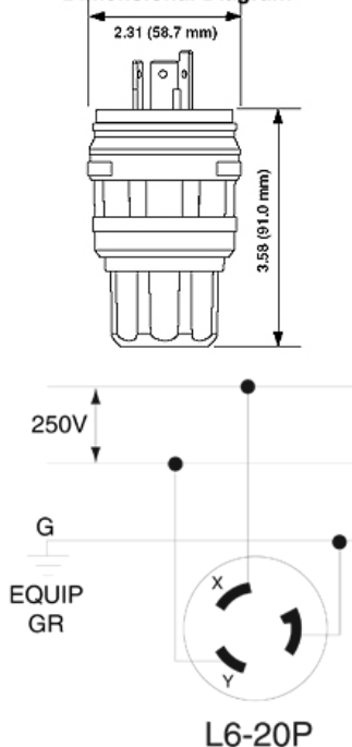
Dimensional Diagram
