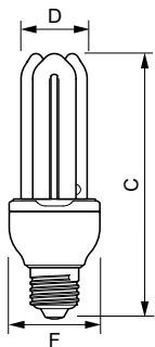
Economy Stick 18W CDL E27 220-240V
