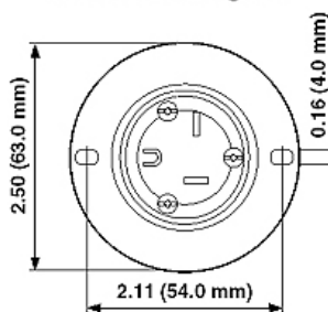
Dimensional Diagram
